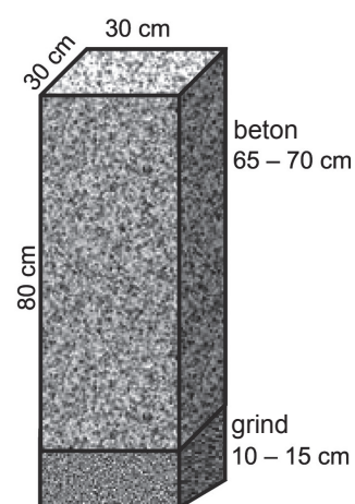
FUNDERING
